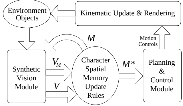
Figure 6. The revised sense-plan-control loop for dynamic environments.
