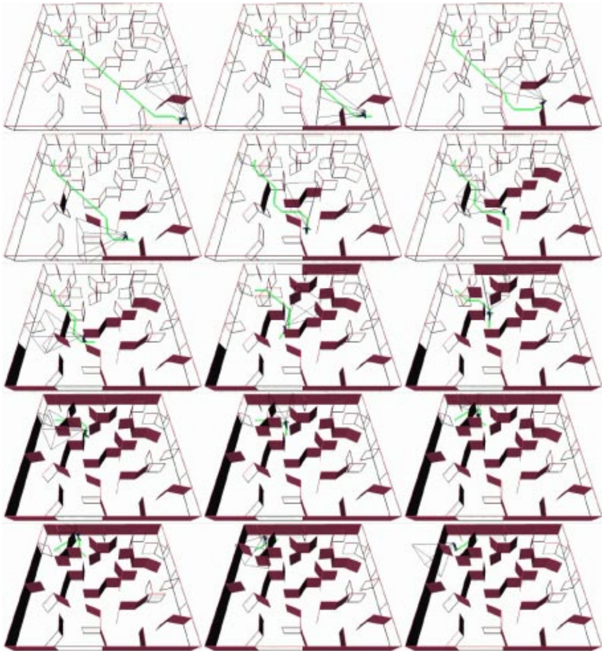
Figure 12. Snapshots of a character exploring an unknown maze environment. Objects rendered solid are those contained in \mathcal{M} , while those rendered wireframe are unknown. The top-left image shows the initial frame with the character given the task of navigating from the bottom-right corner to the top-left corner of the maze. A portion of the character's viewing frustum, along with the current path is also shown.
