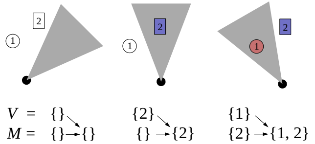
Figure 4. Updating \mathcal{M} in static environments
