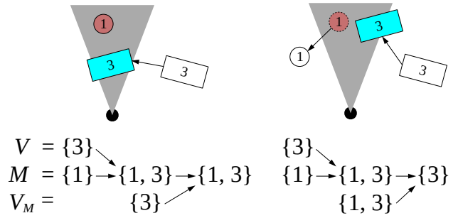
Figure 7. “Obscured” vs. “Missing” scenarios requiring \mathcal{V}_M in order to distinguish between them and update \mathcal{M} properly.
