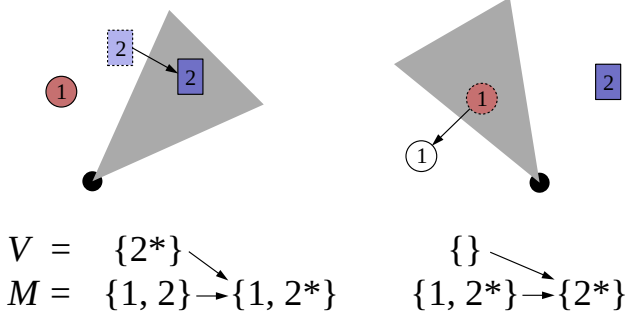
Figure 5. Updating \mathcal{M} in dynamic environments
