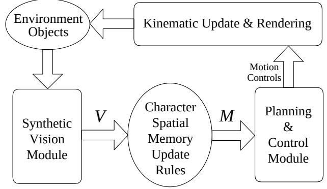
Figure 3. The basic sense-plan-control loop for static environments.
